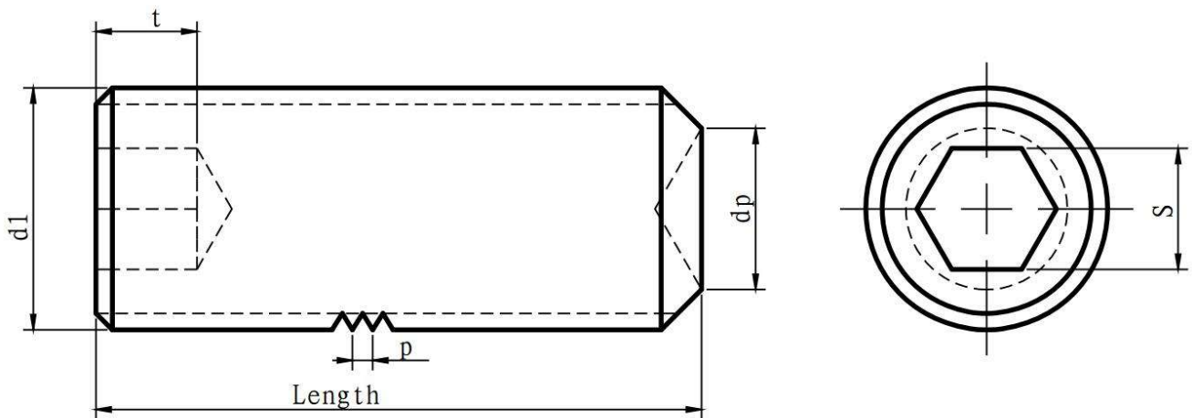
DIN 916 HEXAGON SOCKET SET SCREW WITH CUP POINT SIZE SPECIFICATION
